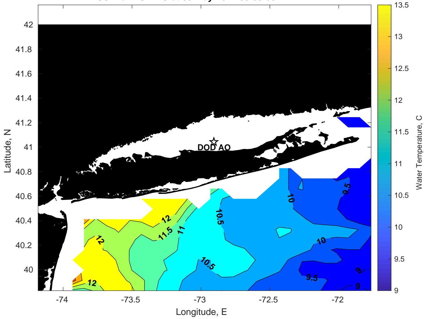
SST for DOD AO at 03-May-2024 00:00:00
